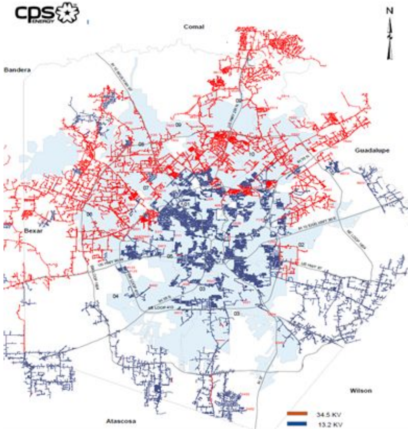
Circuits Used for Load Shed
